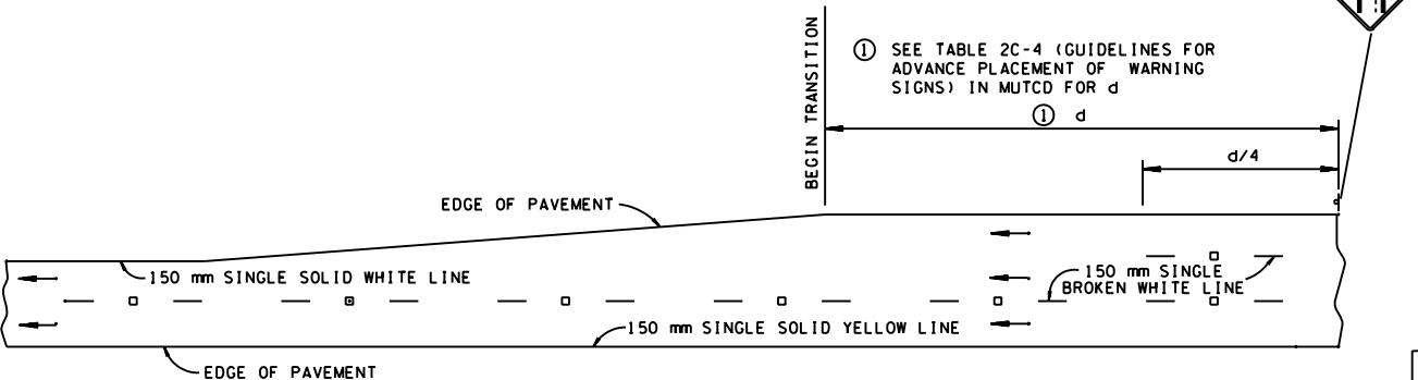
TYPICAL SHOWING ENDING OF ADDITIONAL LANE
