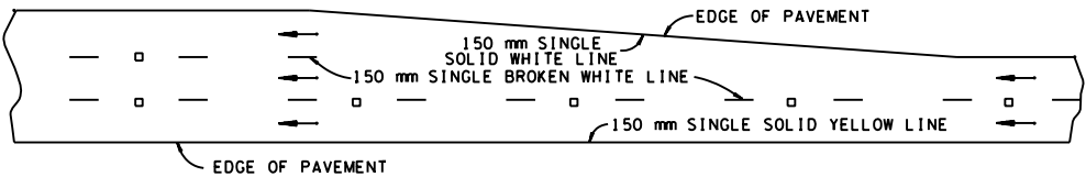
TYPICAL SHOWING BEGINNING OF ADDITIONAL LANE
